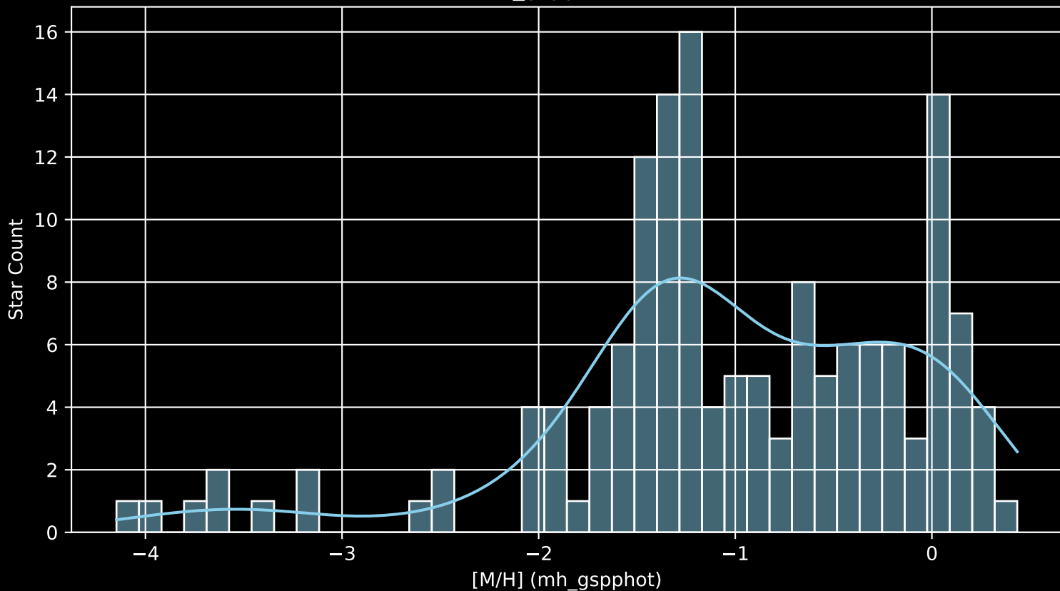
APOGEE DR17 Field: [291-00-C [M/H] (mh_gspphot) (n= 149)
