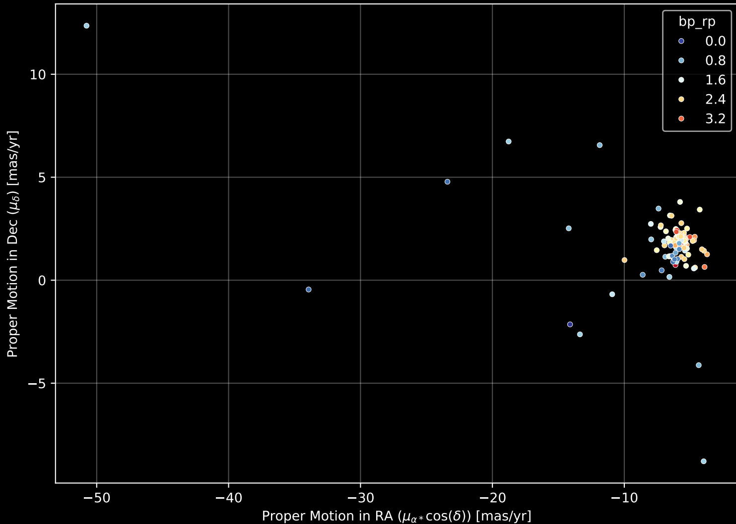
APOGEE DR17 Field: [291-00-C] Proper Motion Diagram (n= 149)
