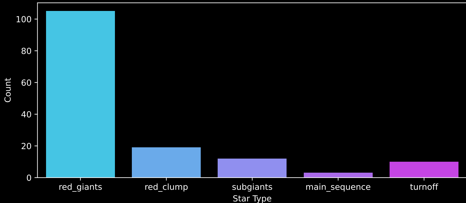
APOGEE DR17 Field: [291-00-C] Count plot of Star Type
