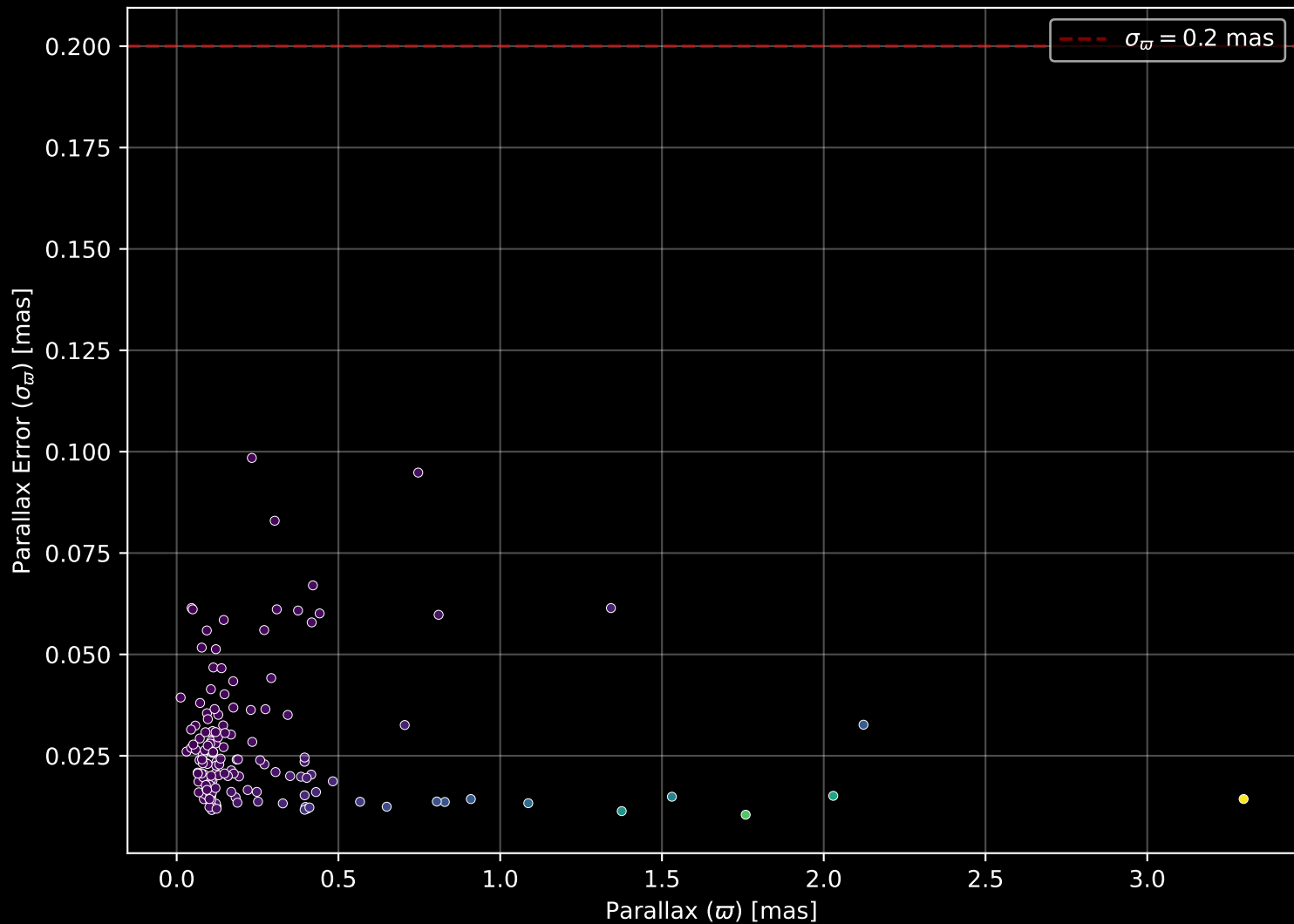
APOGEE DR17 Field: [291-00-C] Parallax Quality (n= 149)
