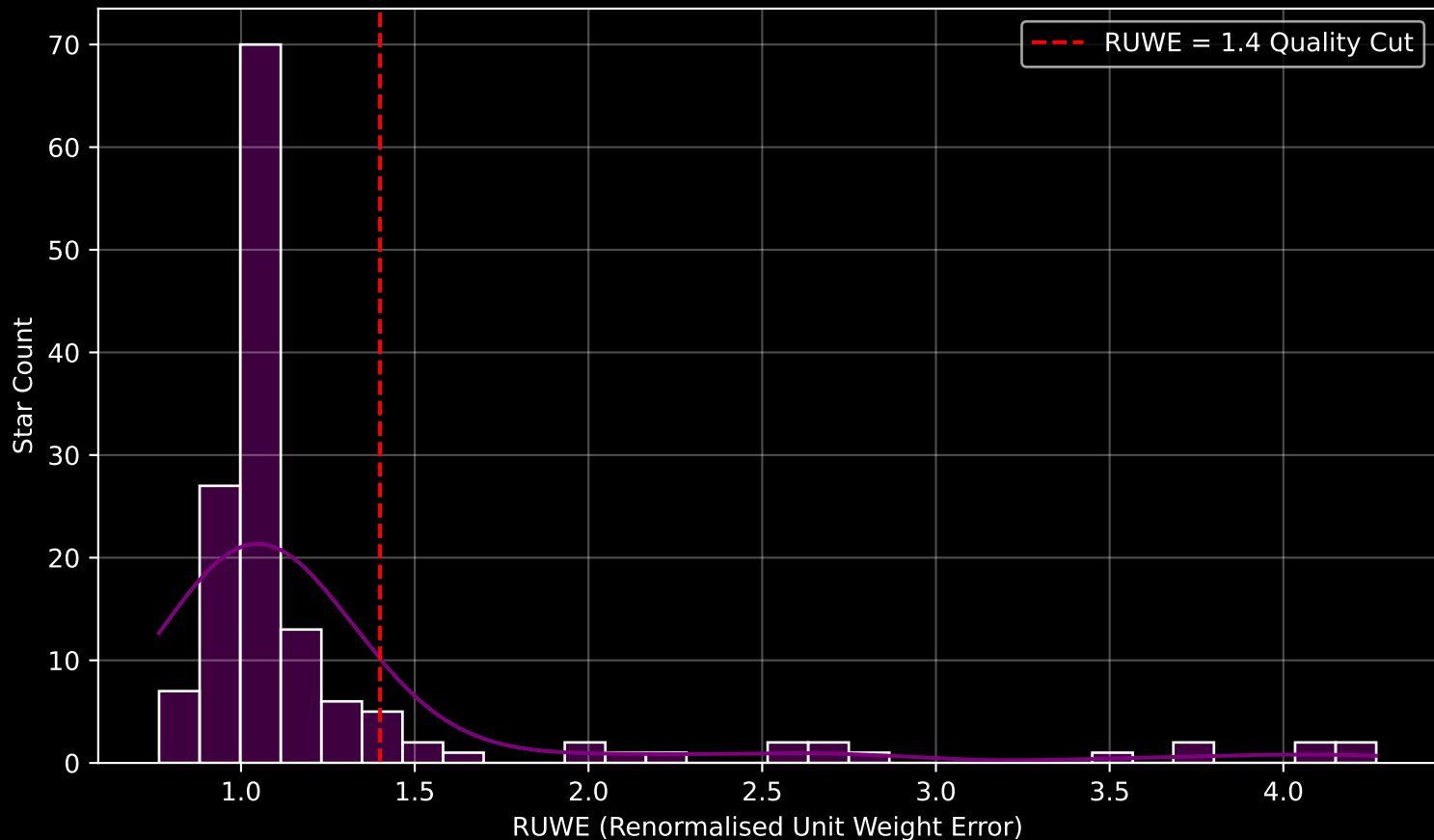
GAPOGEE DR17 Field [291-00-C] RUWE Distribution (n= 147)
