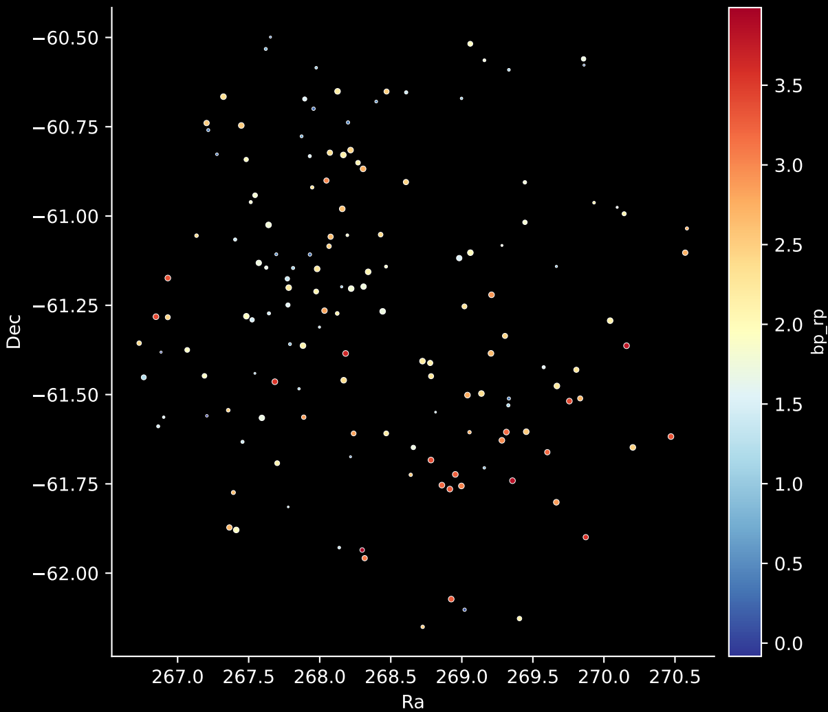
APOGEE DR17 Field: [291-00-C] Stars: 149
